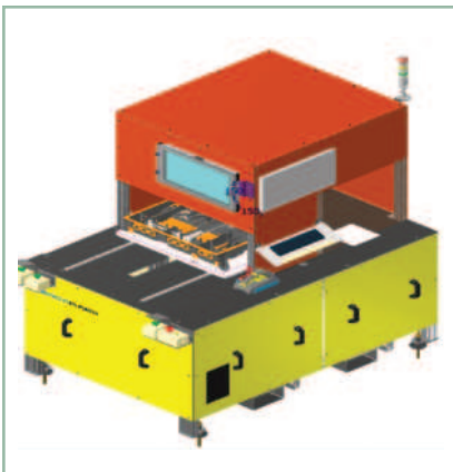
Laser marking
