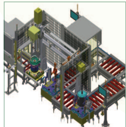
Stator insertion
